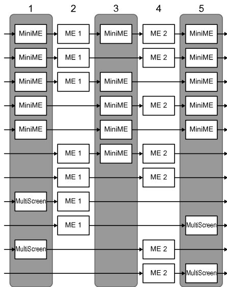
Figure 7: Re-Entry for MiniME™ Mode Timing Windows
