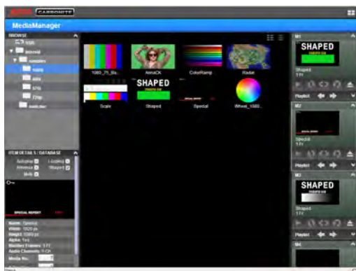
Figure 21: MediaManager Window
