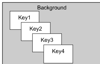
Figure 20: Key Priority
