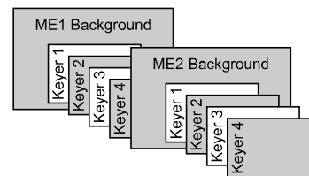
Figure 5: Video Layering
