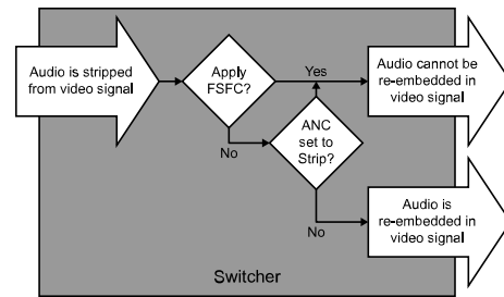
Figure 4: Audio Flow Through the Switcher
