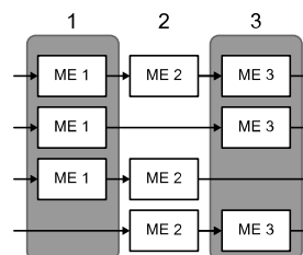
Figure 6: Re-Entry for 3 ME Mode Timing Windows
